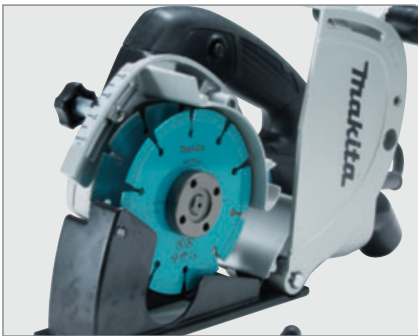
Aluminium blade case designed to allow for easy blade replacement
